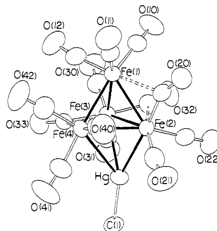
Figure 7. ORTEP diagram of [\text{Fe}_4(\text{HgCH}_3)(\text{CO})_{13}]^- ( 6 (tetrahedron)) with thermal ellipsoids at the 50% probability level. Carbonyl carbons are designated in a manner analogous to the oxygens to which they are attached.
