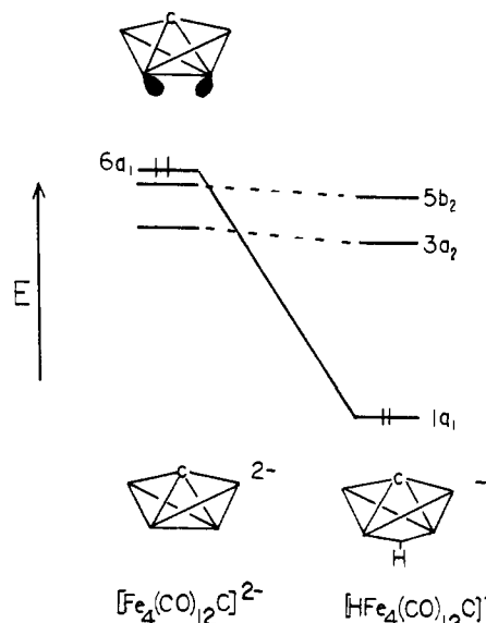
Figure 1. Schematic energy level diagram for [Fe_4(CO)_{12}C]^{2-} and [HFe_4(CO)_{12}C]^- . For complete details see ref 13.
