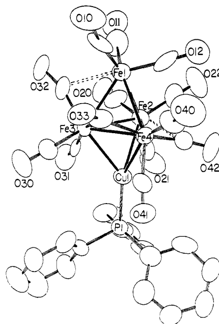
Figure 6. ORTEP diagram of [\text{Fe}_4(\text{CuPPh}_3)(\text{CO})_{13}]^- ( 5a ) with thermal ellipsoids at the 50% probability level. Carbon atoms are designated in a manner analogous to the oxygens to which they are attached.
