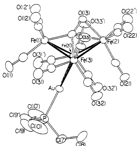
Figure 2. ORTEP diagram of [Fe 4 (AuPEt 3 )(CO) 13 ] - (3a) with thermal ellipsoids at the 50% probability level. Carbonyl carbons are designated in a manner analogous to the oxygens to which they are attached.
